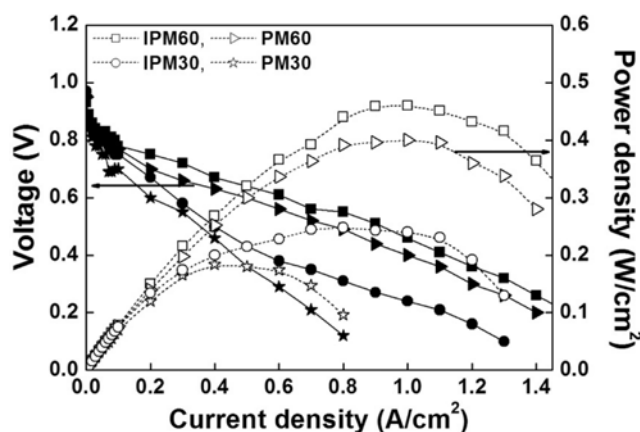
Fig. 4. Single-cell performance.
